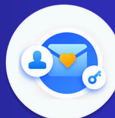
AI INTEGRATION
